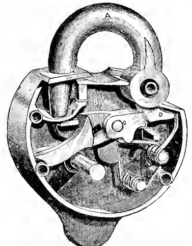
Fig. 2772. RAILROAD PADLOCK.
